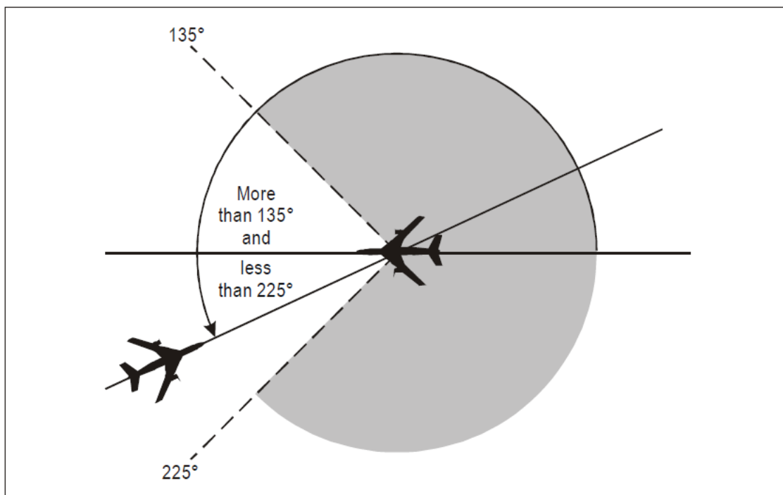
Figure 5-8. Aircraft on reciprocal tracks (see 5.4.2.1.5 b))
