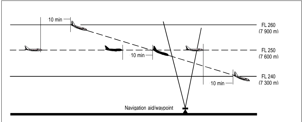
Figure 5-17B. Ten-minute separation between aircraft descending and on same track (see 5.4.2.2.1 b))
