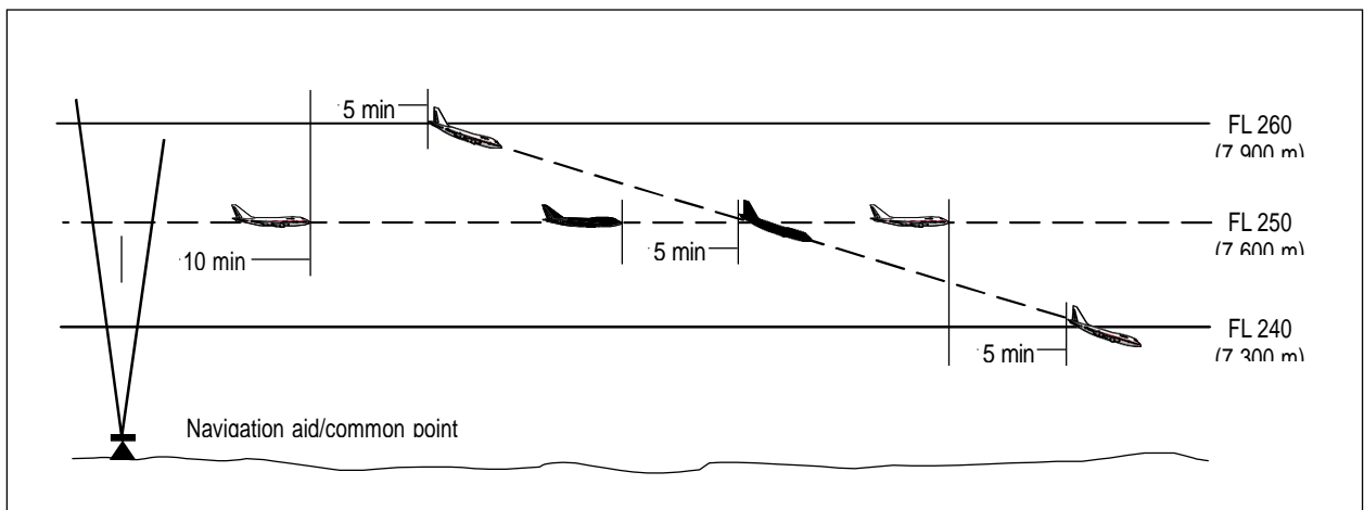
Figure 5-18B. Five-minute separation between aircraft descending and on same track (see 5.4.2.2.1 c) 2))
