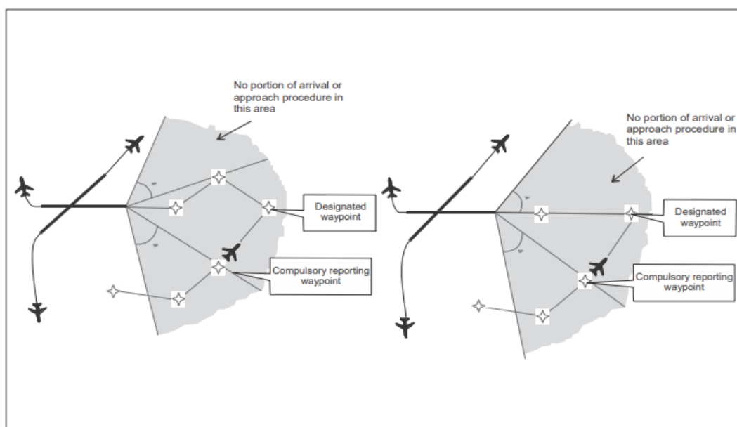
Figure 5-41. Examples of arrival protection area
