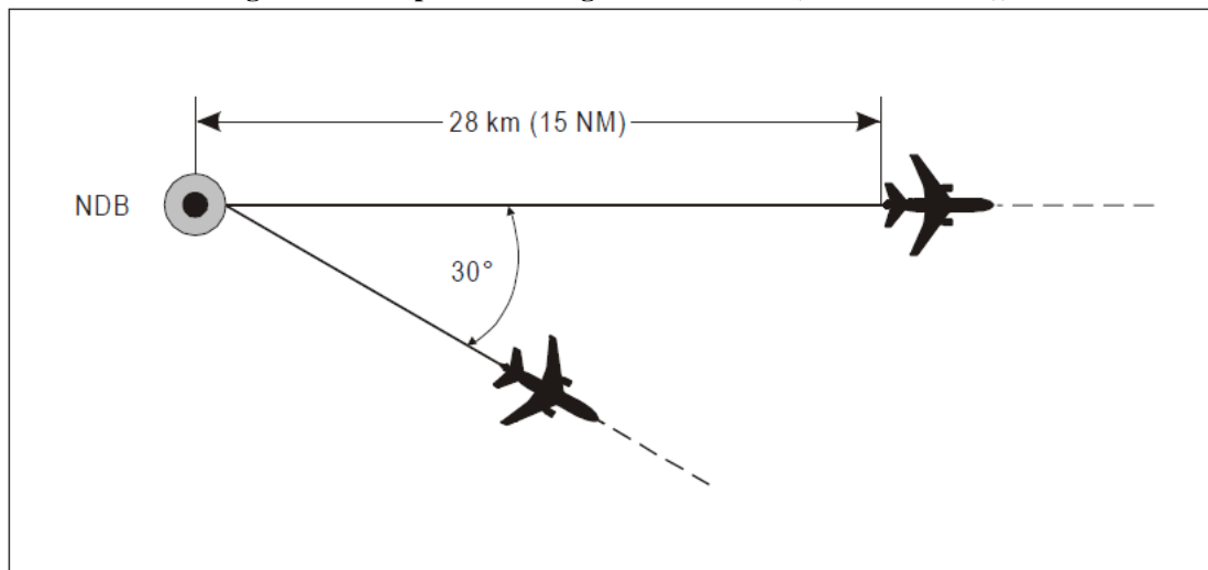
Figure 5-5. Separation using the same NDB (see 5.4.1.2.1.2 b))
