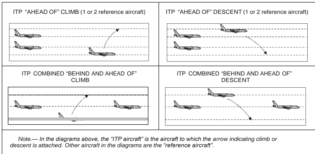
Figure 5-29. ITP flight level change scenarios (see 5.4.2.7.3)
