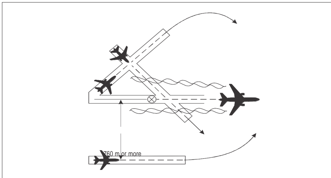
Figure 5-43. Wake turbulence separation for crossing aircraft(see 5.8.3.1 c) and d) and 5.8.3.2 c) and d))
