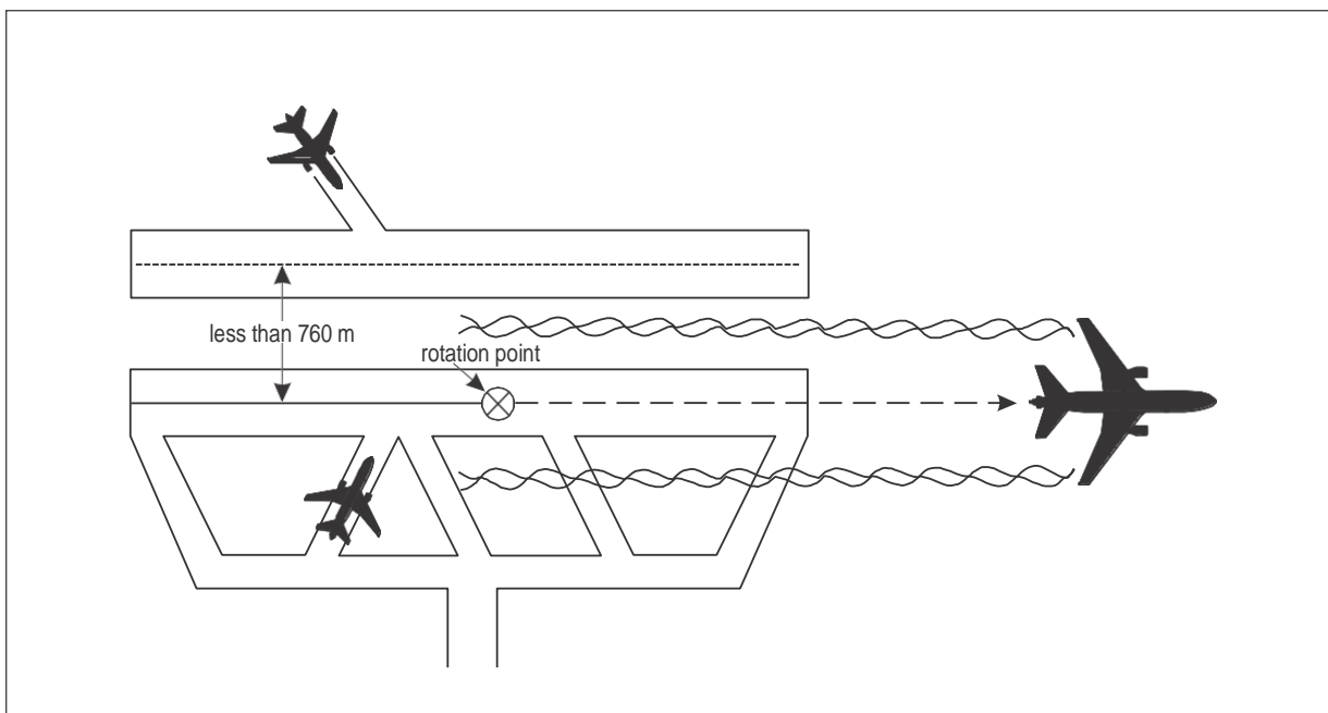
Figure 5-44. Wake turbulence separation for following aircraft(see 5.8.3.3 and 5.8.3.4)
