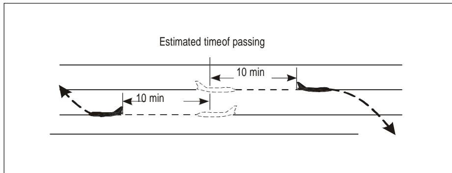
Figure 5-21. Ten-minute separation between aircraft on reciprocal tracks (see 5.4.2.2.3)
