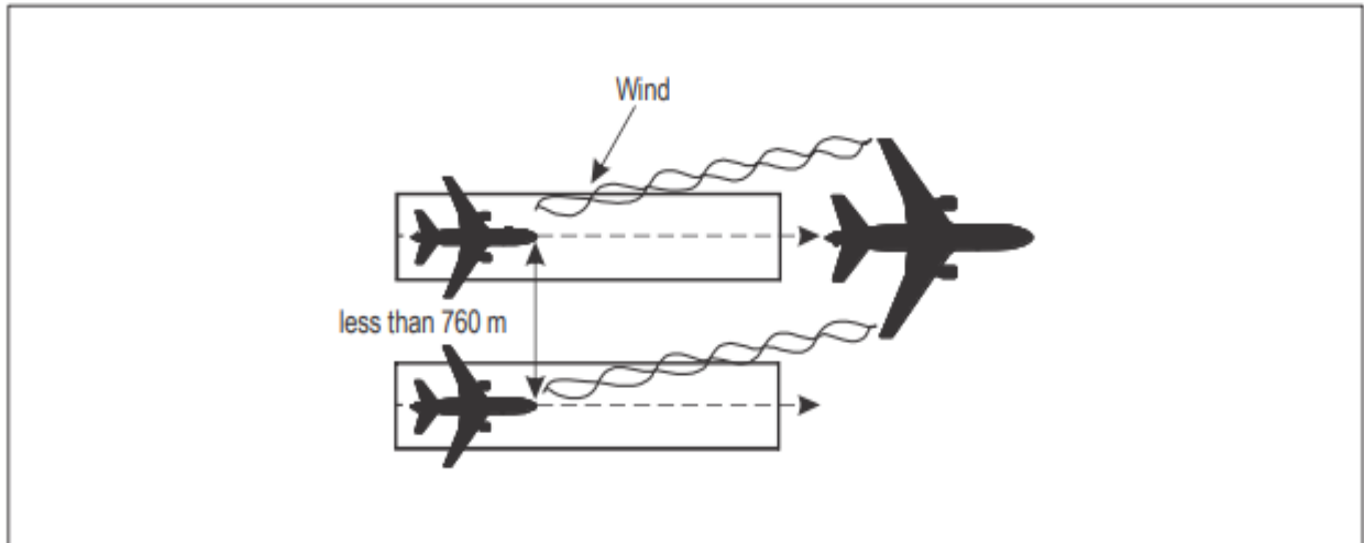
Figure 5-42. Wake turbulence separation for following aircraft (see 5.8.3.1 a) and b) and 5.8.3.2 a) and b))
