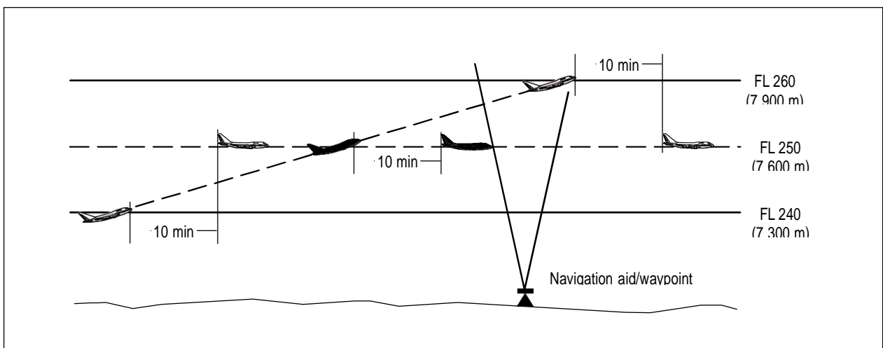
Figure 5-17A. Ten-minute separation between aircraft climbing and on same track (see 5.4.2.2.2.1 b)
