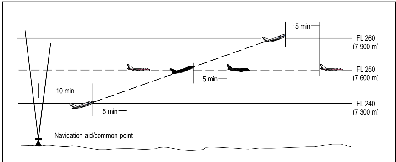
Figure 5-18A. Five-minute separation between aircraft climbing and on same track (see 5.4.2.2.1 c) 2))
